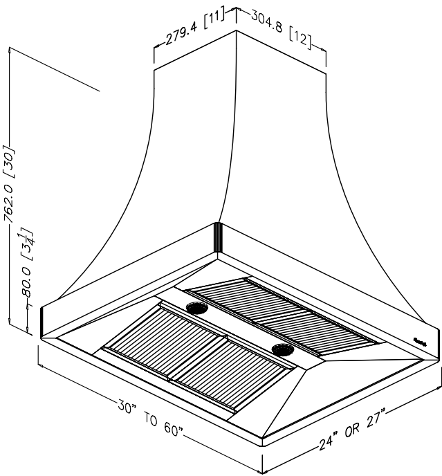
ISO VIEW
