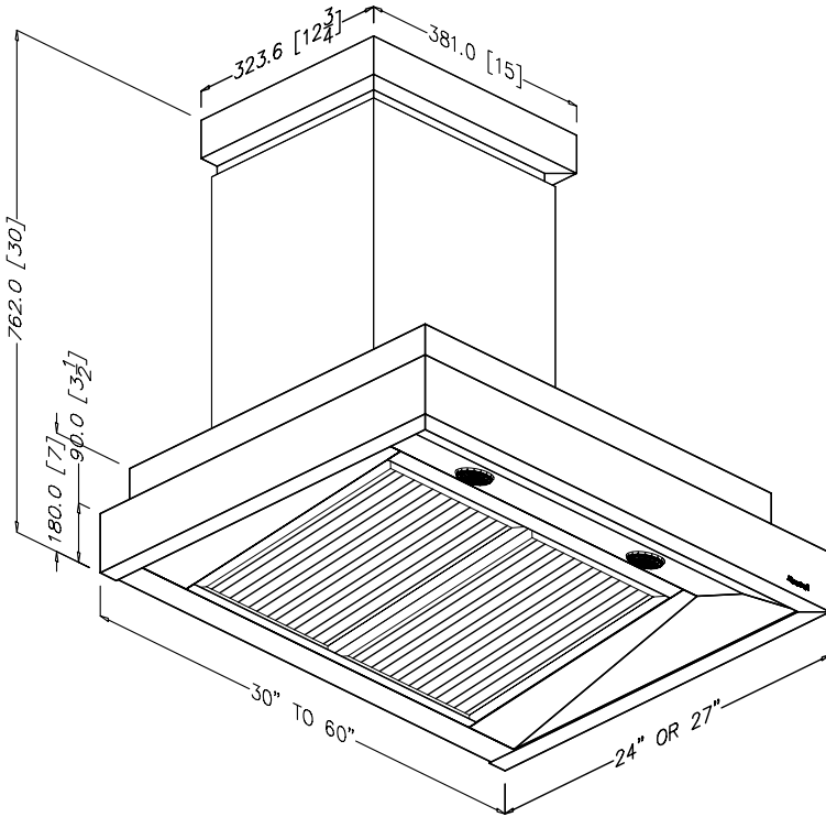
ISO VIEW
