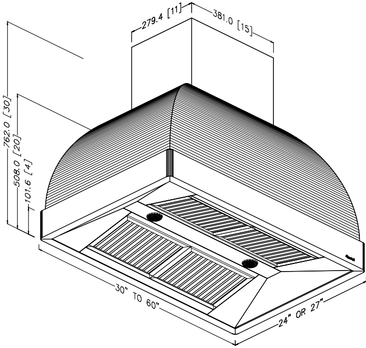
ISO VIEW
