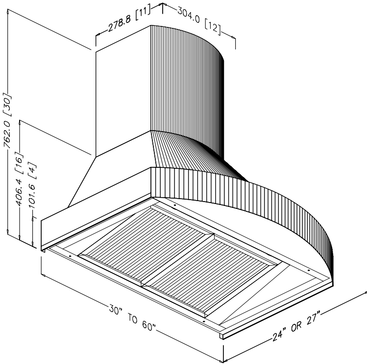
ISO VIEW
